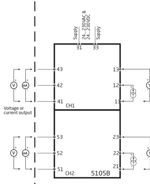
5105B Associated apparatus parameters
