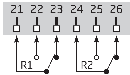
Relais
