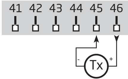
2-Draht-Messumformer
