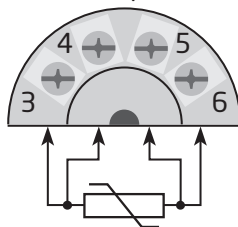
RTD, 4-проводн.
